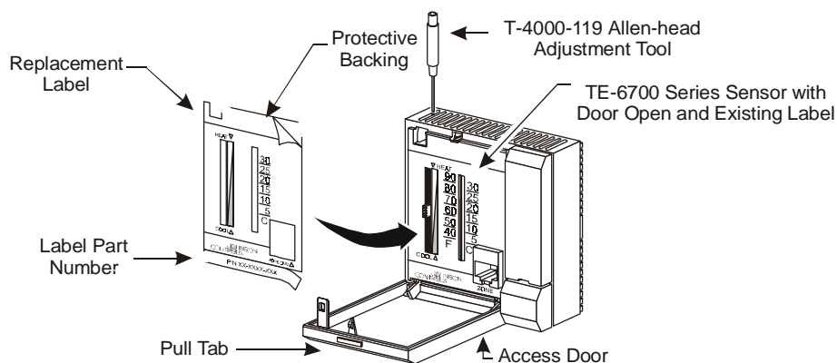
Figure 1: Affixing a Label onto the Temperature Sensor
