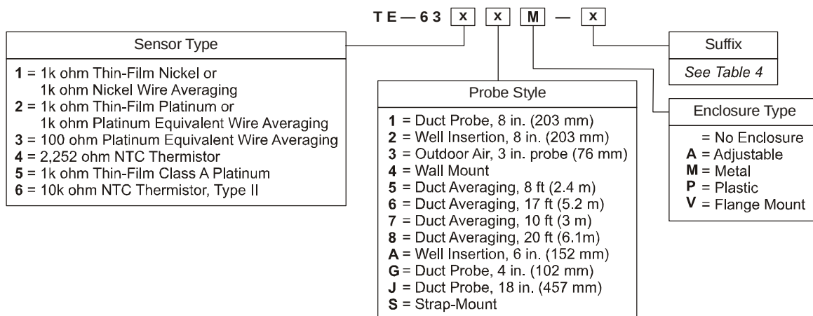
Figure 5: Ordering Template
