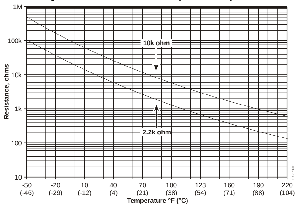
Figure 3: Thermistor Sensor Response
