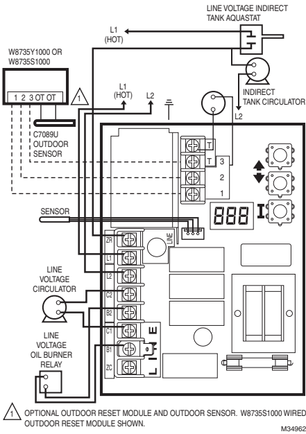
Fig. 9. L7224U single heat zone with indirect water tank and circulators. Optional outdoor reset module.
