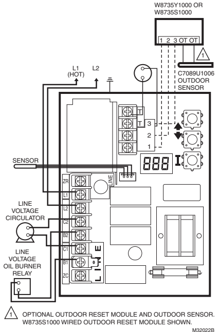
Fig. 8. L7224U single zone connections.
