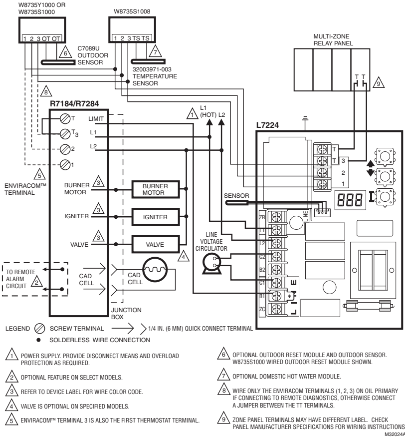
Fig. 11. L7224U multizone system with Outdoor Reset and Domestic Hot Water Modules (indirect tank applications).
